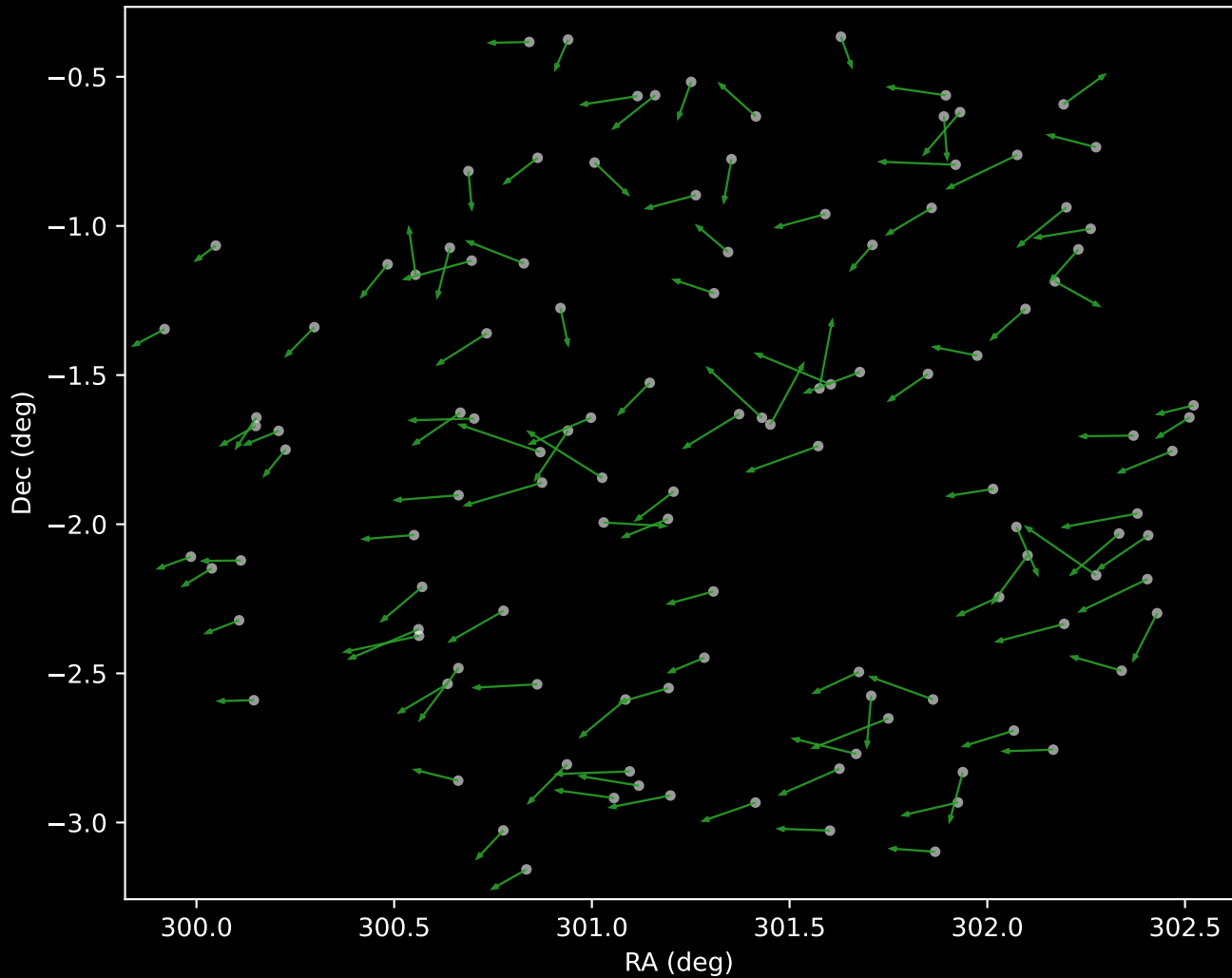
APOGEE DR17 Cluster 4 Proper Motion Vectors (n=118)
