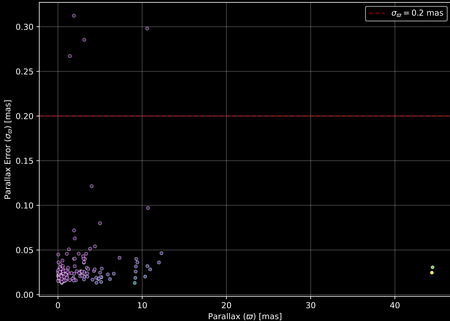
APOGEE DR17 Field: [320+60] Parallax Quality (n= 184)
