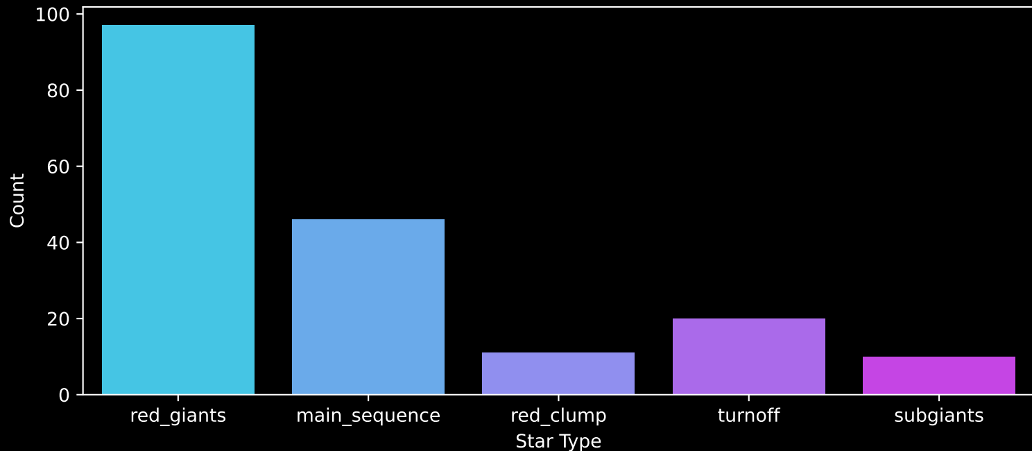
APOGEE DR17 Field: [320+60] Count plot of Star Type
