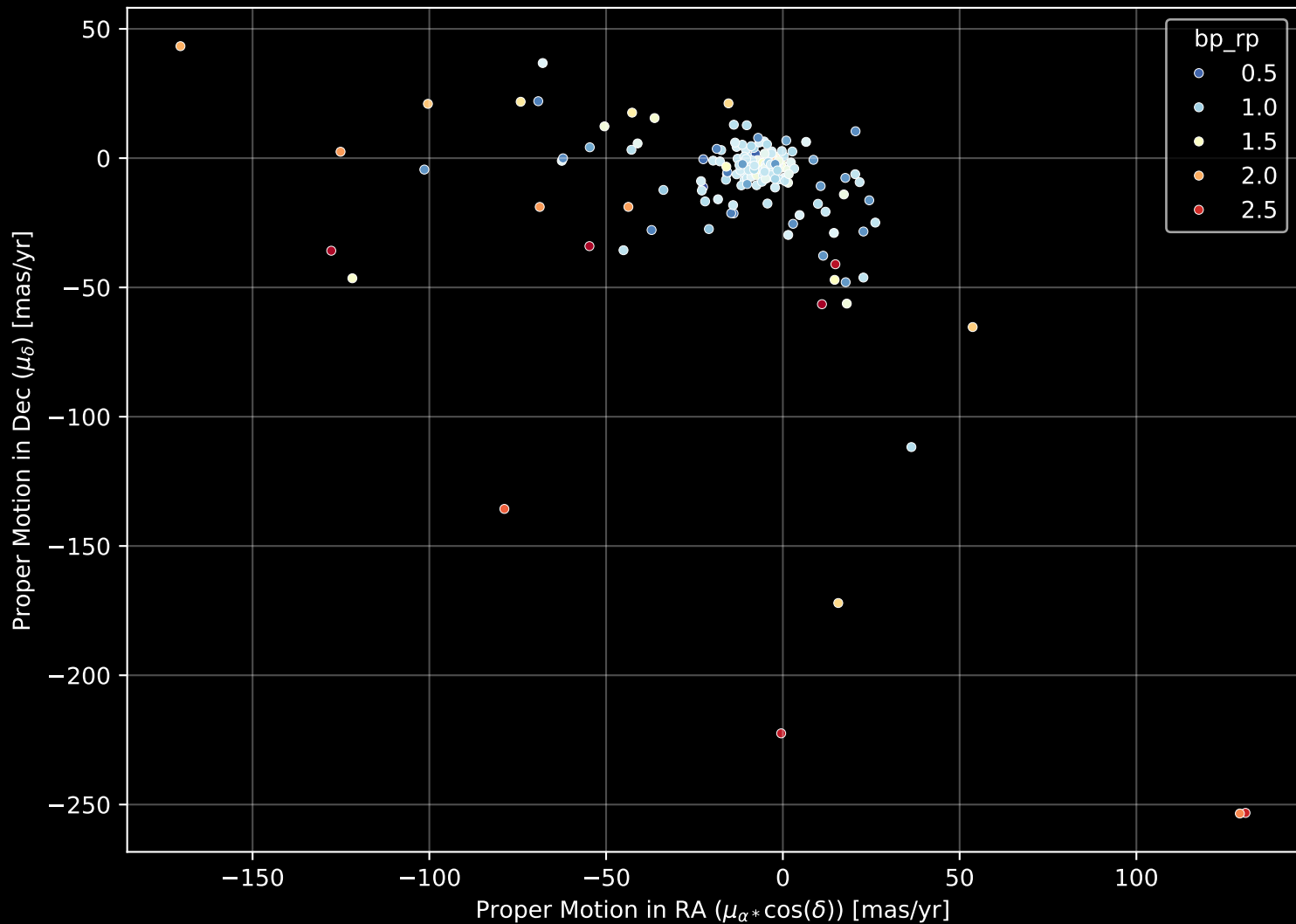
APOGEE DR17 Field: [320+60] Proper Motion Diagram (n= 184)
