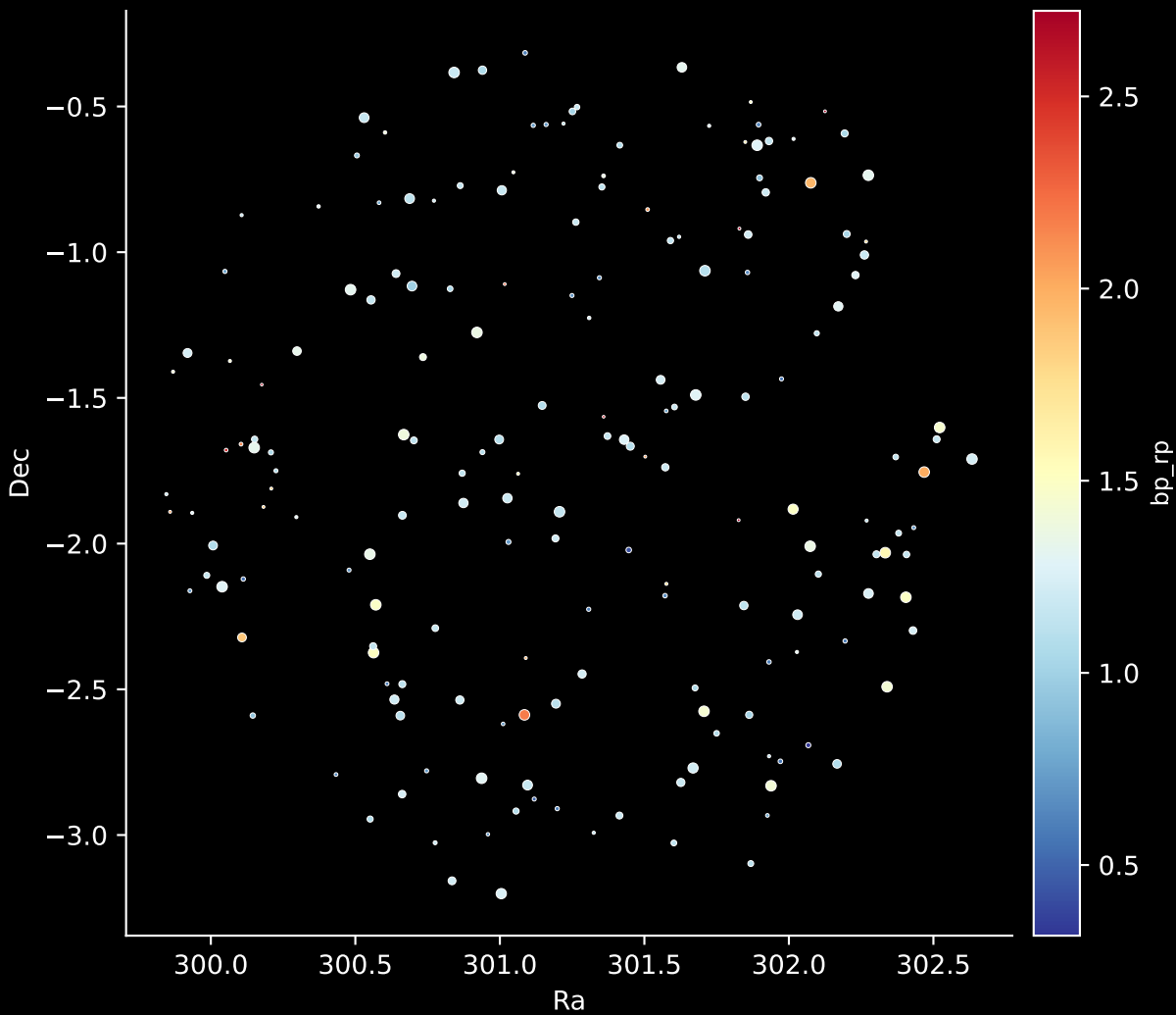
APOGEE DR17 Field: [320+60] Stars: 184
