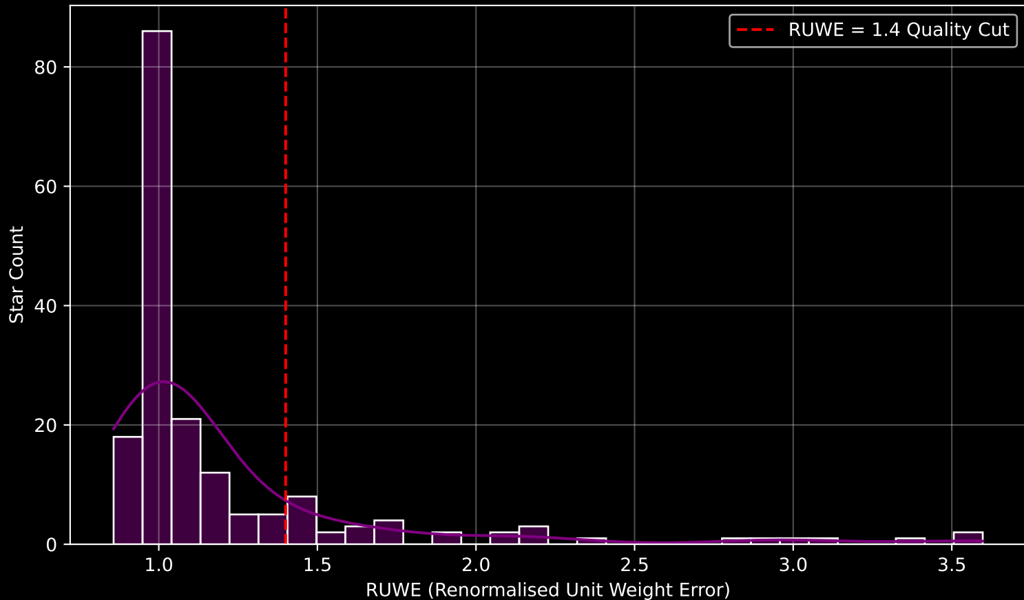
GAPOGEE DR17 Field [320+60] RUWE Distribution (n= 179)
