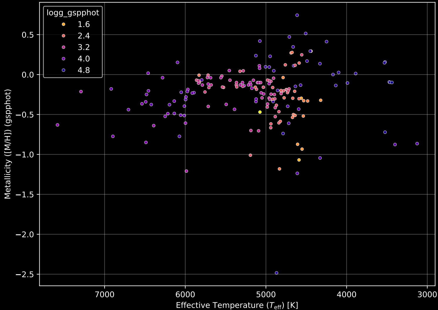
APOGEE DR17 Field: [320+60] Stellar Population Parameters (n= 184)
