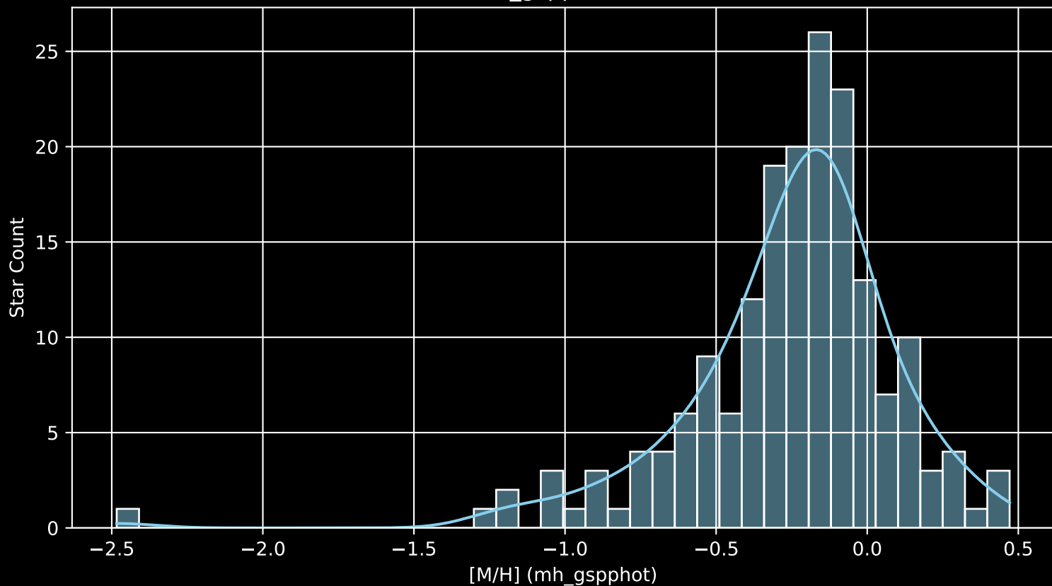
APOGEE DR17 Field: [320+60 [M/H] (mh_gspphot) (n= 182)
